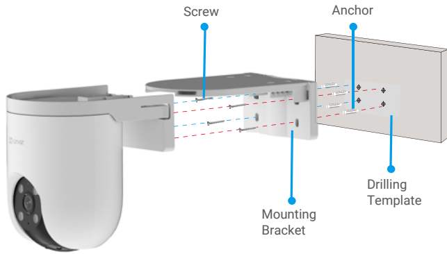
Fig. 2 Wall Mount
